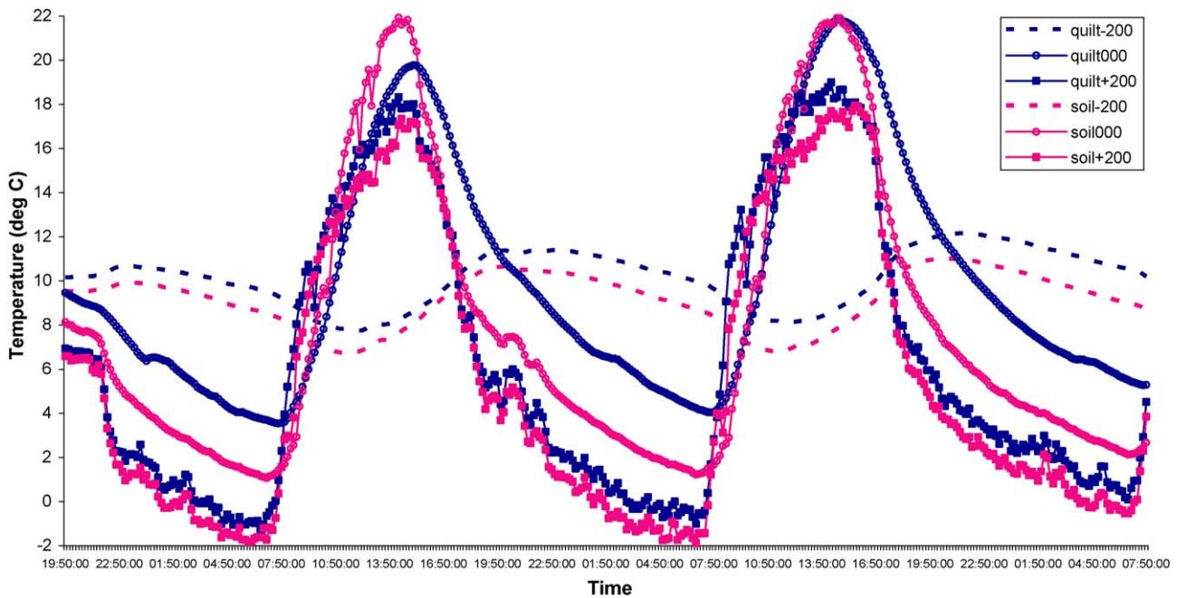
Fig. 5. Average air, surface and soil temperatures measured at the Waihopai Valley Road vineyard, New Zealand with and without plastic quilt sheeting [4].
